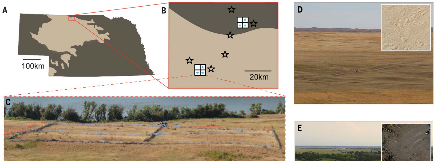
Fig. 1. Experimental site and environmental variation in the Sand Hills region of Nebraska. (A) Map of Nebraska showing the Sand Hills region (light color) and location of the enclosure experiment. (B) Map of the replicate enclosures (squares) and sampling locations for mice introduced to the enclosures (stars) used in the experiment (table S8). Light blue asterisks indicate the six enclosures used; we did not introduce mice to the fourth enclosure at either site. (C) Enclosures are shown at the light site in Sand Hills habitat (truck for scale). (D and E) Typical habitat is shown on the Sand Hills (D, light habitat) and off the Sand Hills (E, dark habitat); insets show typical soil substrate.
